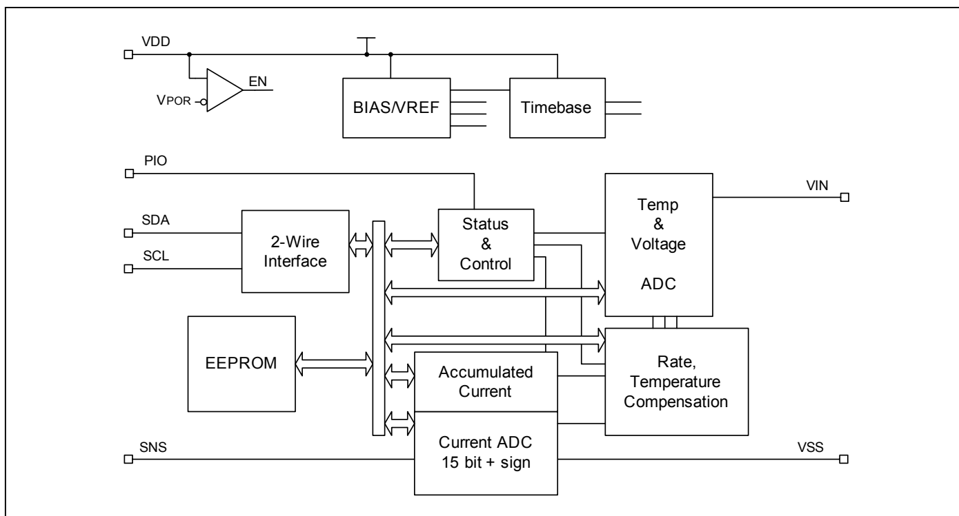
Figure 2. Block Diagram
